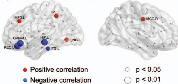
Figure 6. Effect of IQ on regional nodal properties. The significant positive and negative correlation between IQ and regional nodal parameters are shown in red and blue, respectively. The significances of p < 0.05 and p < 0.01 (uncorrected) are indicated by spheres in small and big size, respectively. For a description of the abbreviations, see Table S1. doi:10.1371/journal.pone.0055347.g006
