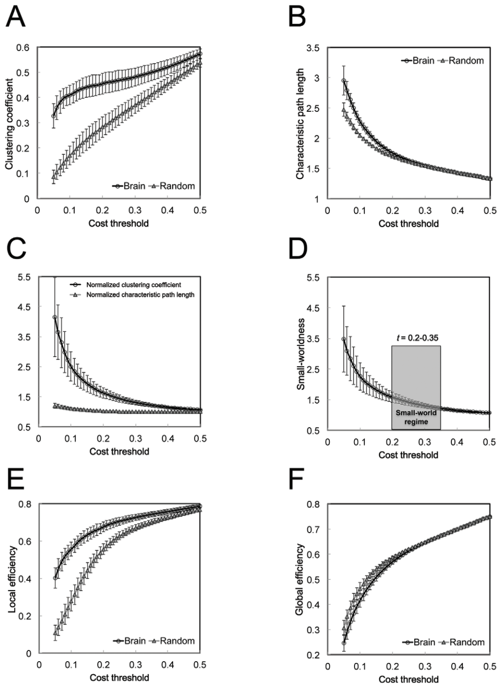
Figure 1. Global network properties. (A) The clustering coefficient and (B) the characteristic path length are shown as a function of cost thresholds and compared to the matched random networks. (C) The normalized clustering coefficient, the normalized characteristic path length, and (D) the small-worldness are shown as a function of cost thresholds. Note that the small-world regime of cost threshold adopted in this study was from 0.2 to 0.35. (E) The local efficiency and (F) the global efficiency are shown as a function of cost thresholds and compared to the matched random networks. Error bars indicate standard error in all subjects. doi:10.1371/journal.pone.0055347.g001
