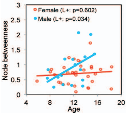
Figure 5. Age-by-sex interaction on regional nodal properties. The significant age-by-sex interactions on regional nodal parameters are shown. The correlation between age and regional nodal parameters are shown in female and male groups, respectively. For a description of the abbreviations, see Table S1. doi:10.1371/journal.pone.0055347.g005
