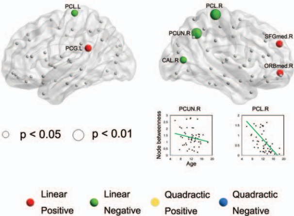
Figure 3. Effect of age on regional nodal properties. Significant linear positive, linear negative, quadratic positive, and quadratic negative correlations are indicated by red, green, yellow, and blue spheres, respectively. The significances of p < 0.05 and p < 0.01 (uncor-
