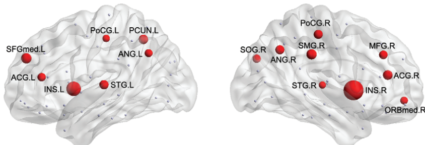
Figure 2. Global hubs in functional brain networks. Global hubs are defined as the brain regions with higher values ( > \text{Mean} + \text{SD} ) in any of (A) node degree, (B) node efficiency, and (C) node betweenness. The global hubs are shown in red with node sizes that indicate the values in regional nodal parameters. For a description of the abbreviations, see Table S1. doi:10.1371/journal.pone.0055347.g002
